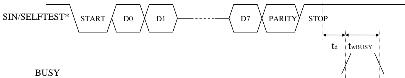
Figure 2. Serial Interface
