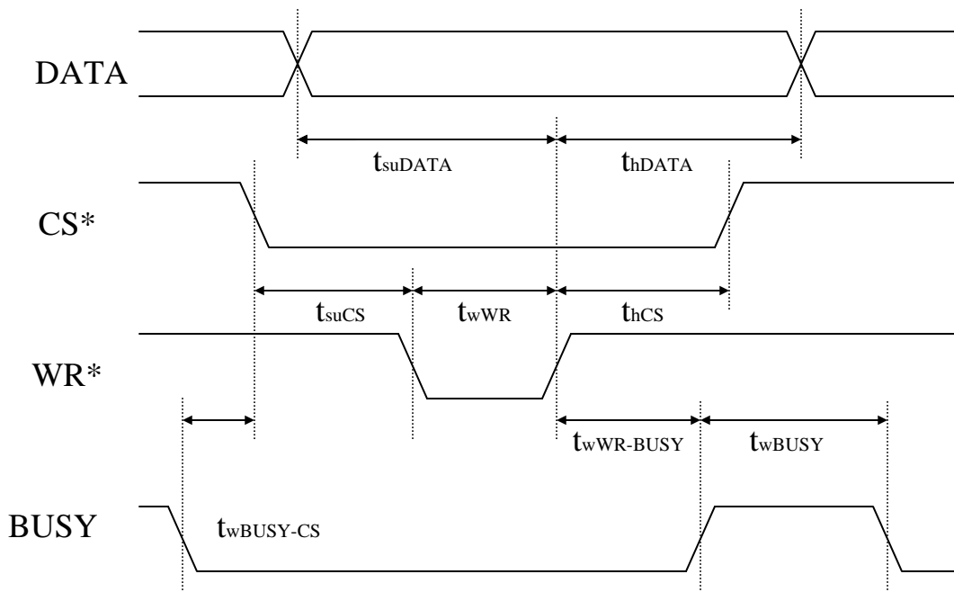
Figure 1. Parallel Interface
